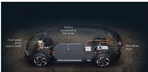
E-GMP - Structure
